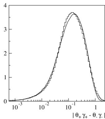
Fig. 7.15: Distribution of the difference of transverse momenta of positive and negative muons (with logarithmic x-scale).
