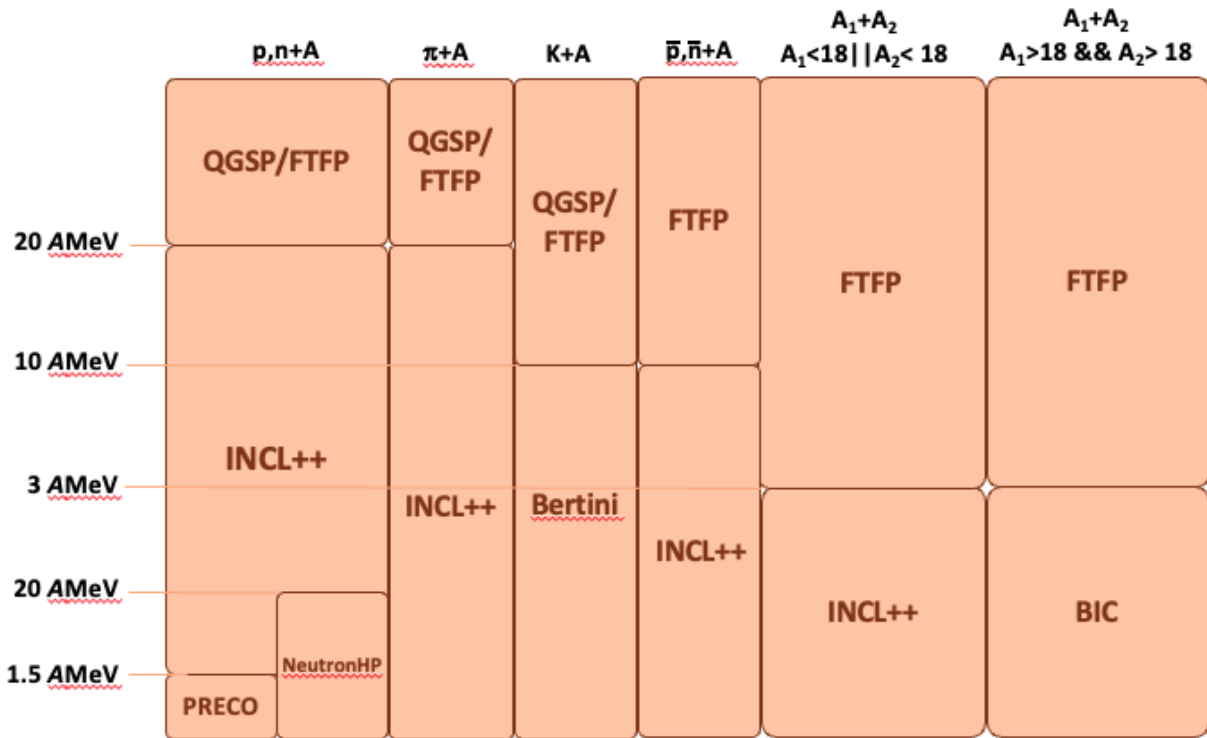
Fig. 27.1: Model map for the INCL++-based physics lists. The first two columns represent nucleon- and pion-induced reactions. The third column represents kaon-induced reactions and the fourth one antinucleon-induced reactions. The last two columns deal with nucleus-nucleus reactions, according to the masses of the partners (below or above A = 18 ).
